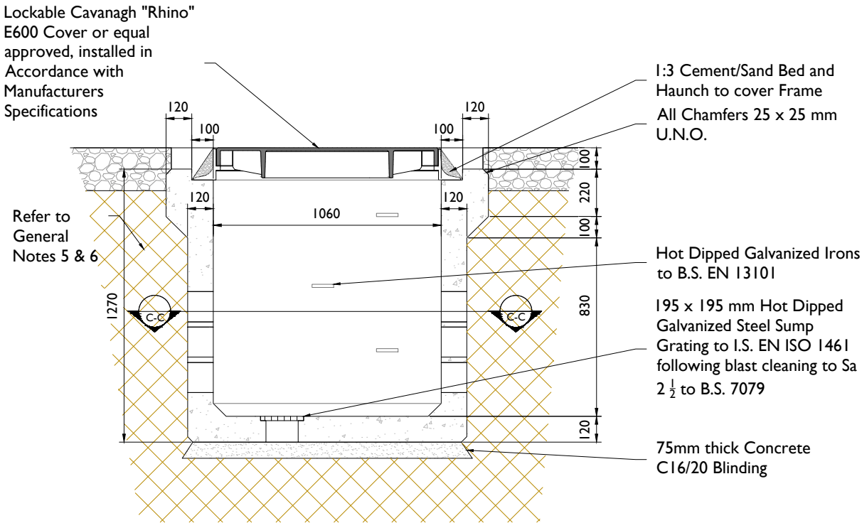
C2 Chamber - Section A-A Scale 1:25
